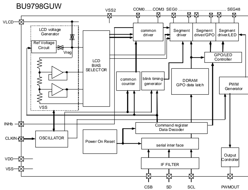
Figure 4. Block Diagram
