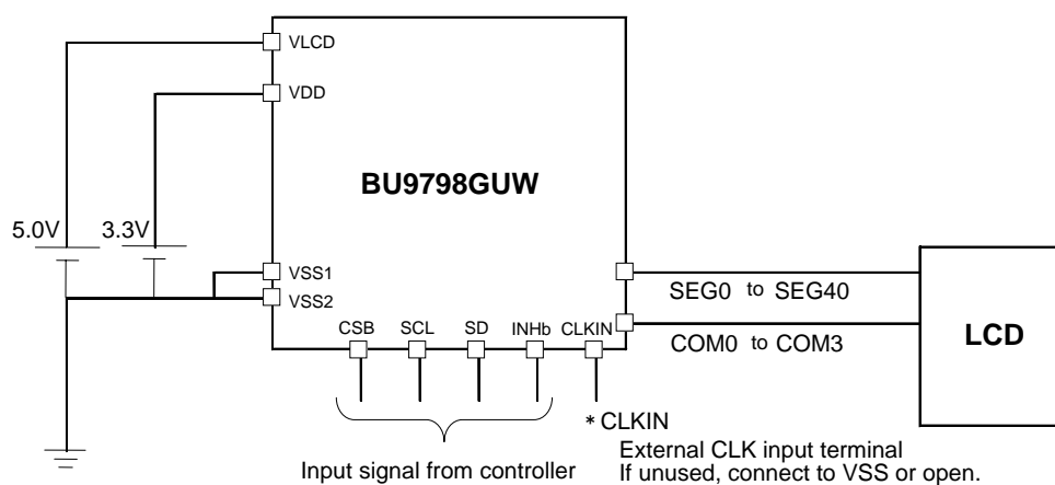
Figure 10. BU9798GUW example of recommended circuit
